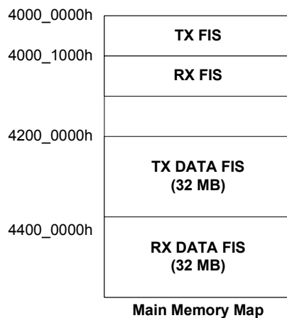
Figure 11 Memory map of Main Memory (DDR2)
