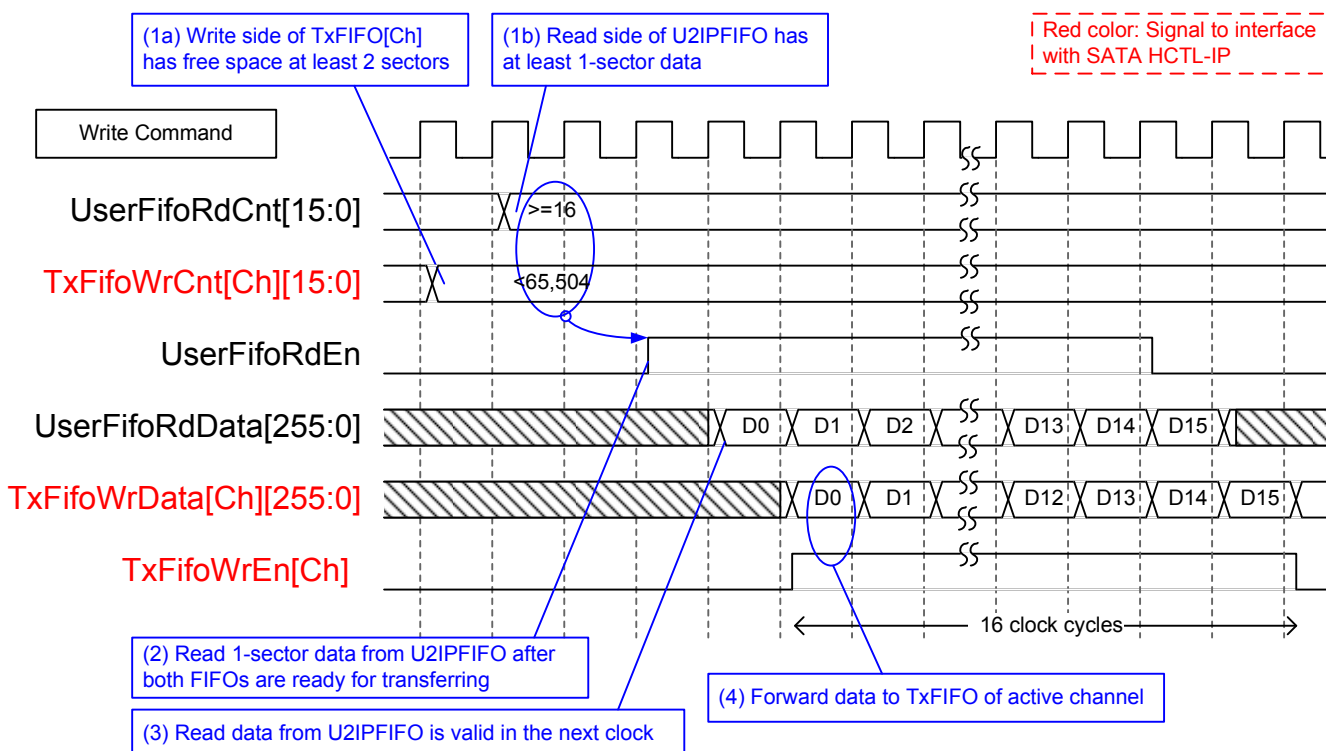
Figure 2-7 Raid0x8 data timing diagram of Write command
