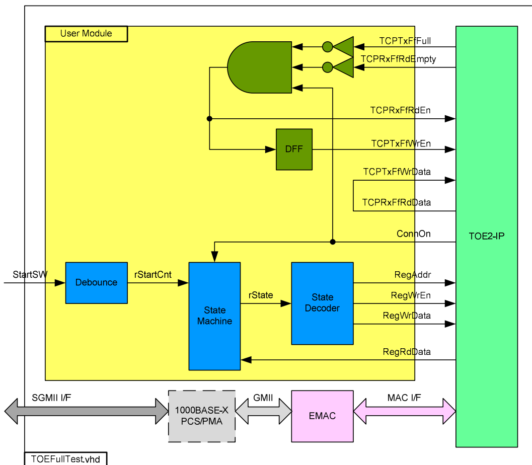
Figure 3 User Module and Test System block diagram
