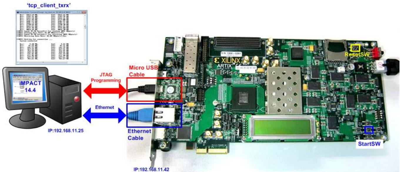
Figure 1 TOE1GIP Demo on Development board
