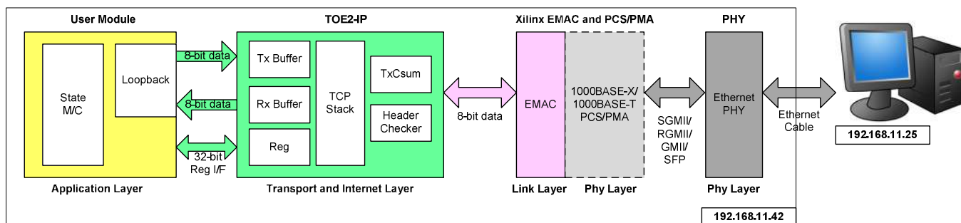
Figure 2 Hardware Architecture in AC701/KC705/VC707/ZC706 reference design
